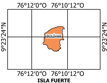
VIENTOS 80 M PROM MULTIANUAL BOLIVAR (m/s)
