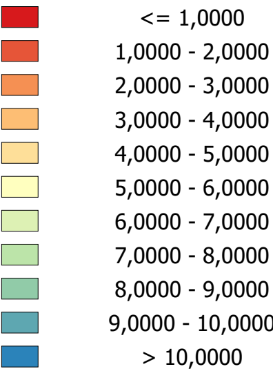
VIENTOS 80 M PROM MULTIANUAL BOLIVAR (m/s)
