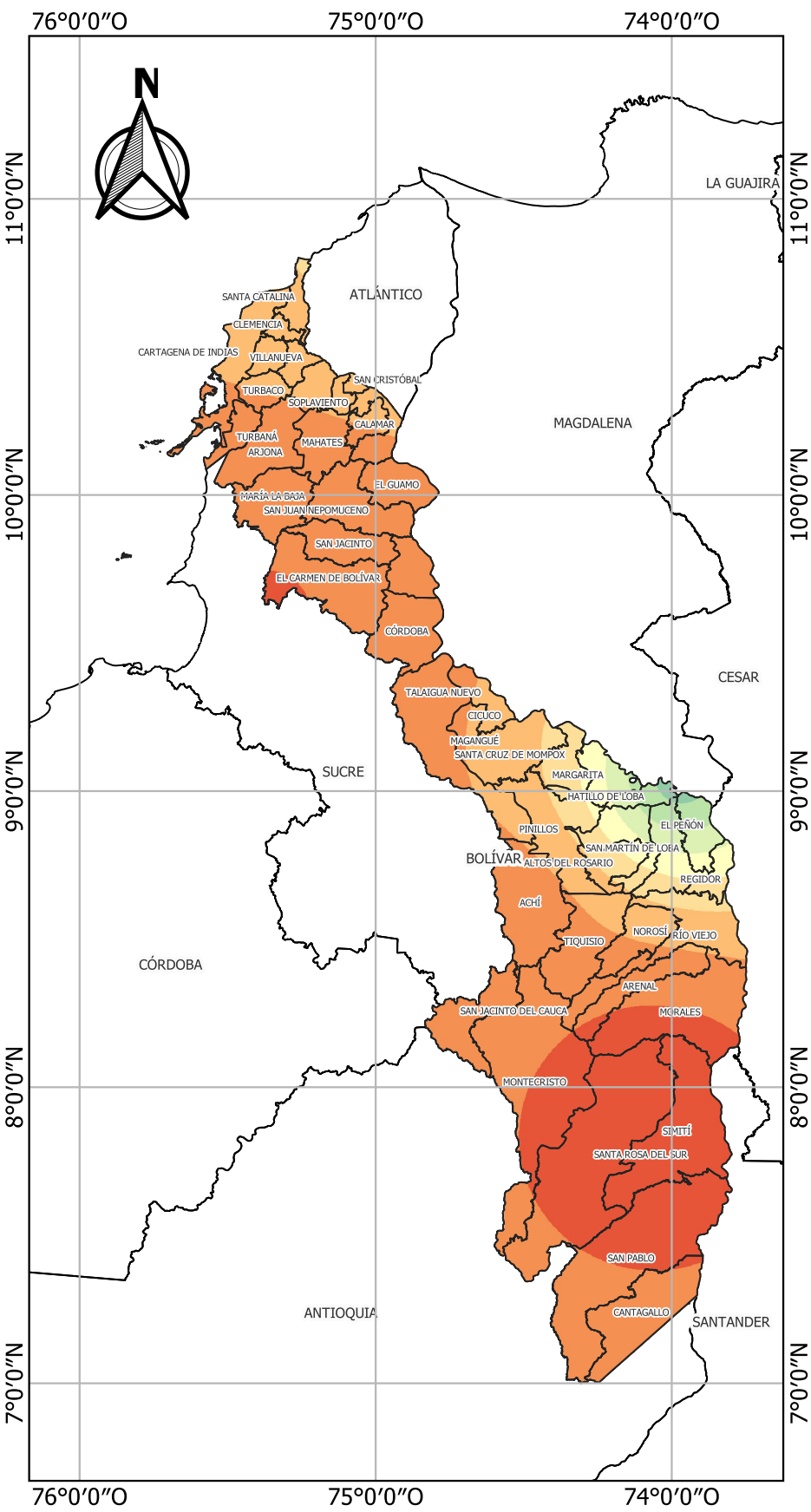
VIENTOS 80 M PROM MULTIANUAL BOLIVAR (m/s)
